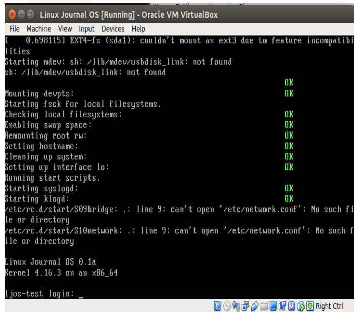
Figure 2. The User Login Prompt
